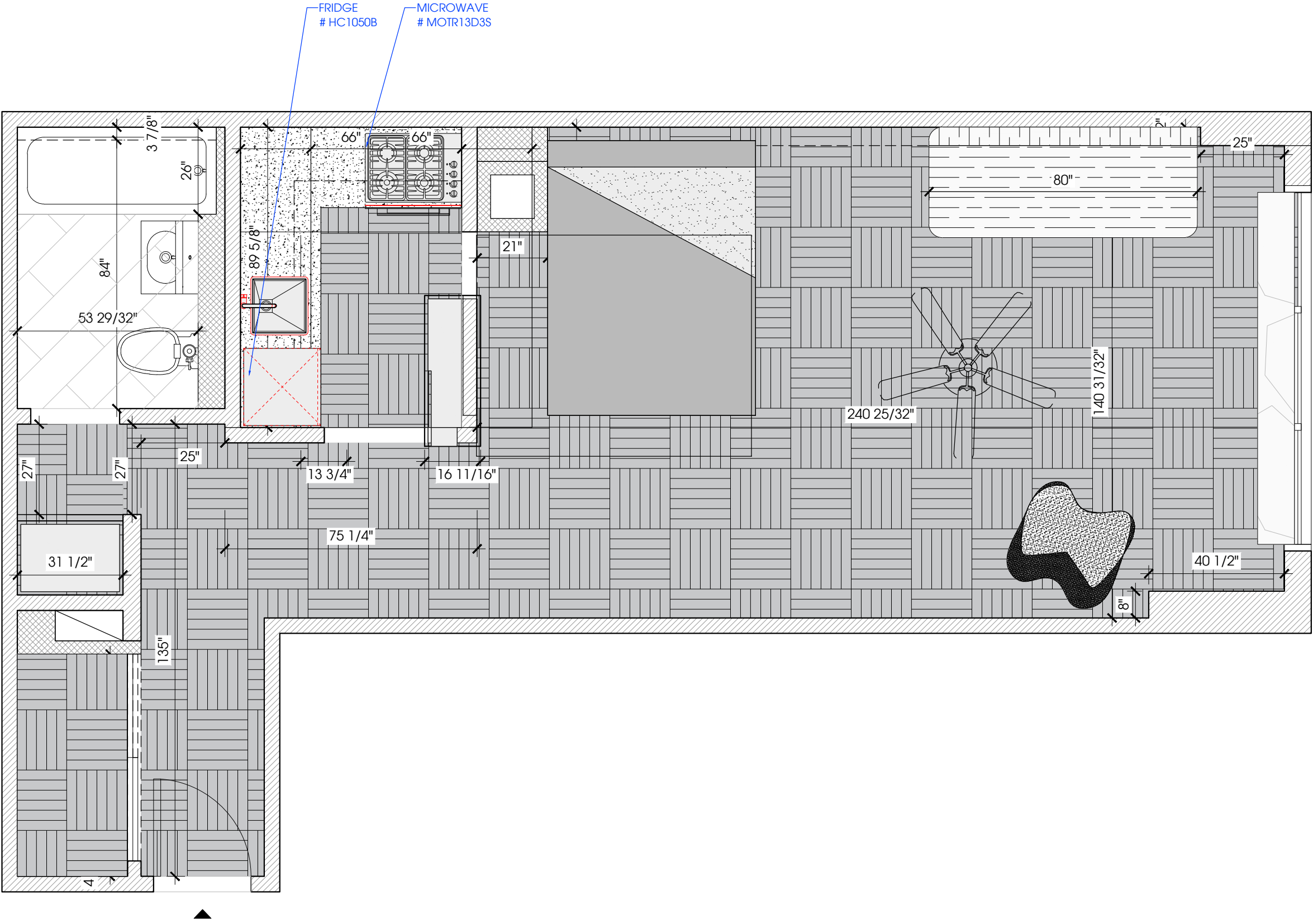
01 PLAN SCALE 3/8"=1' GENERAL LAYOUT
